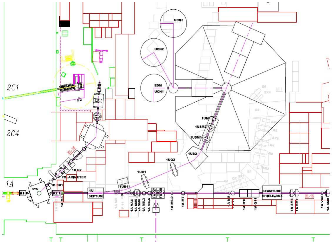
Figure 7: Possible location of the UCN facility in the meson hall. In this scenario, both M11 and M13 would be decommissioned. The beamline layout shown is based on TRIUMF design note TRI-DN-08-3.
