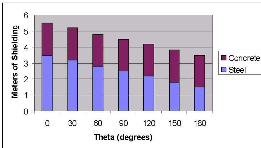
Figure 9: Shielding required for a 40 \mu\text{A} , 500 MeV proton beam incident on a thick tungsten target. The design dose rate is 3 \mu\text{Sv/hr} immediately outside the shielding.
