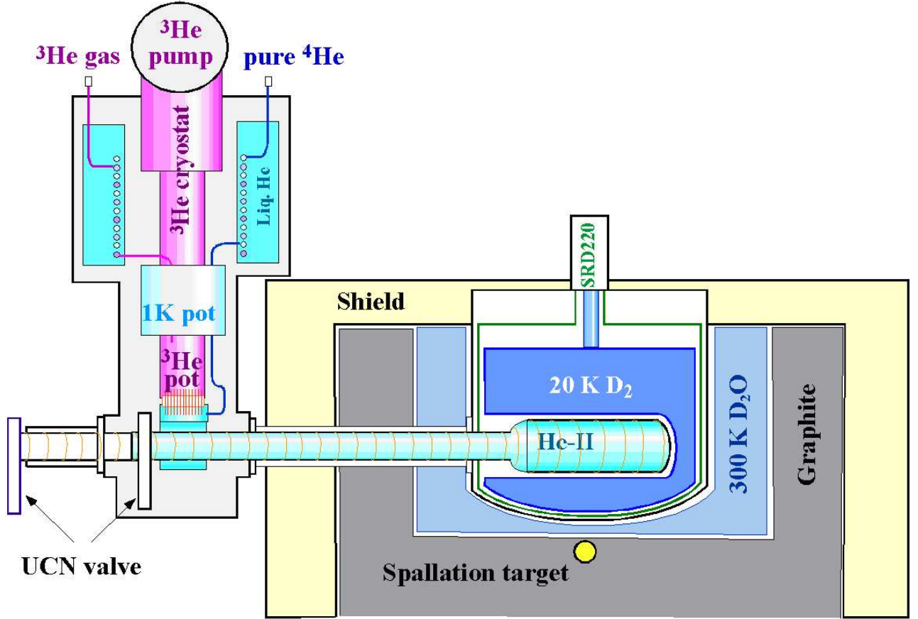
Figure 5: Schematic diagram of the He-II spallation UCN source for TRIUMF.
