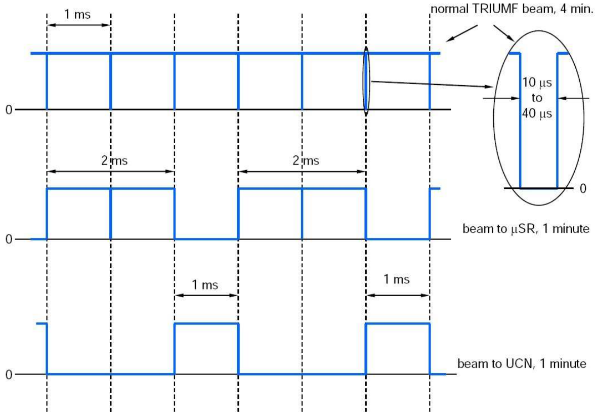
Figure 8: Proposed method of sharing the proton beam between the UCN source and other meson hall users. Every 4 minutes, the UCN source takes a minute of beam in the form of a 1 ms burst every 3 ms. The instantaneous beam current is not affected and the total loss of integrated beam to downstream users is about 7%. The exact details of the time division will depend on what specifications are achievable for the fast kicker magnets.
