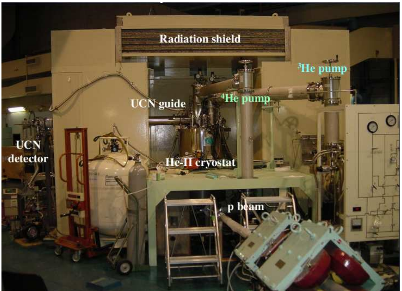
Figure 6: Y. Masuda's UCN source at Research Center for Nuclear Physics, Osaka.
